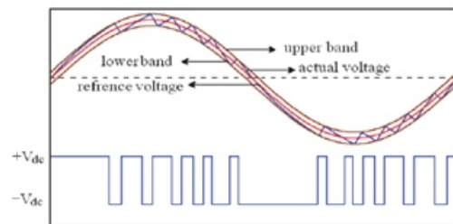
Fig.5 Hysteresis switching pattern
