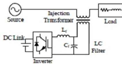
Fig.1. Basic Components of a DVR
