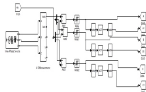
Fig.11 Hysteresis Voltage Controller.
