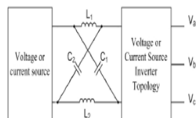
Fig. 6 General Block Diagram of Z-Source Inverter
