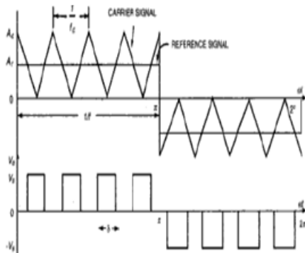
Fig. 7 Multiple Pulse Width Modulation
