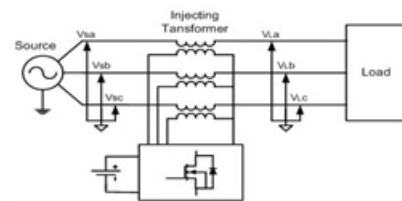
Fig.2. Basic Principle of DVR
