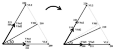
Fig.4. Vector diagram in the first sector of Fig.1 (b) showing the change of the vectors using balanced dc and unbalanced dc assuming v_{C1} < v_{C2} .
