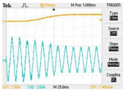
Fig. 18. Battery current CH1 and phase “a” grid current CH2.
