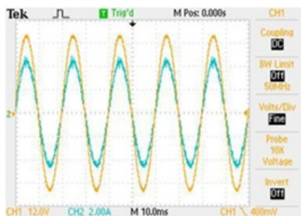
Fig. 19. Phase “a” grid voltage and current waveforms.
