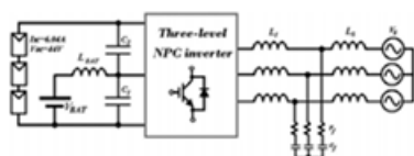
Fig.8. block diagram of the simulated system.
