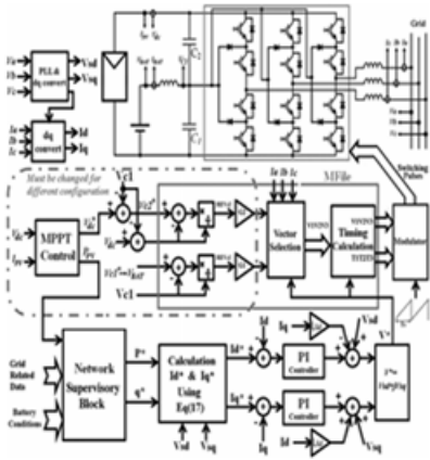
Fig. 7. Control system diagram to integrate PV and battery storage.
