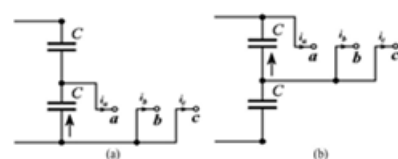
Fig.2. Equivalent circuit and capacitors current with two different short vector. (a) short vector -100,(b) short vector-211.
