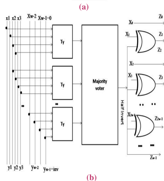
Fig. 1. Encoder architecture scheme I. (a) Circuit diagram. (b) Internal view of the encoder block.
