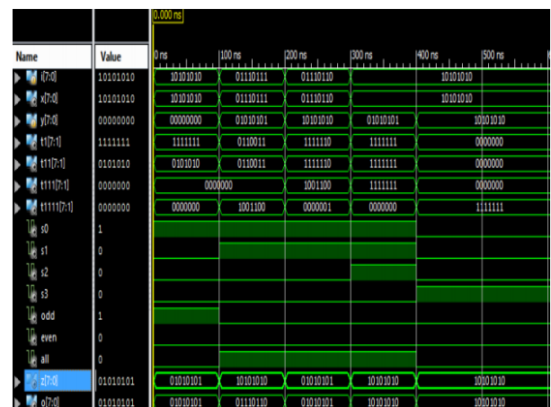
Fig.9. Scheme III Encoder.
