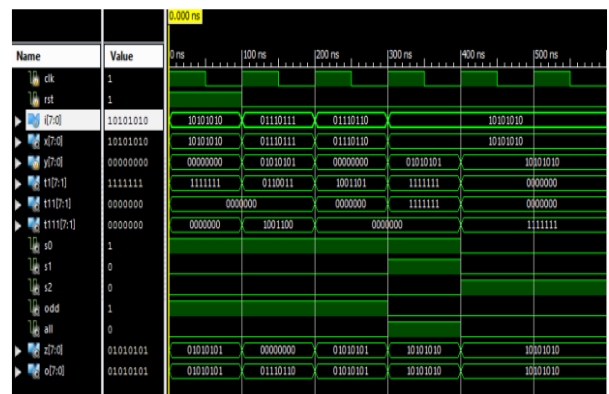
Fig.8. Scheme II Encoder.
