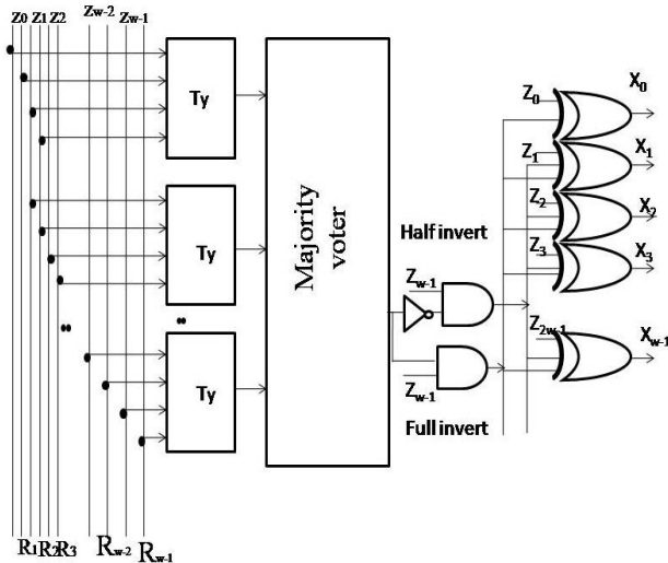
Fig.6. Decoder Architecture Scheme II.
