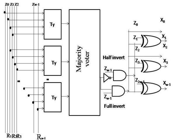
Fig.5. Decoder Architecture Scheme I.
