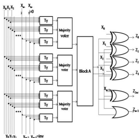
Fig.2. Encoder Architecture Scheme II.
