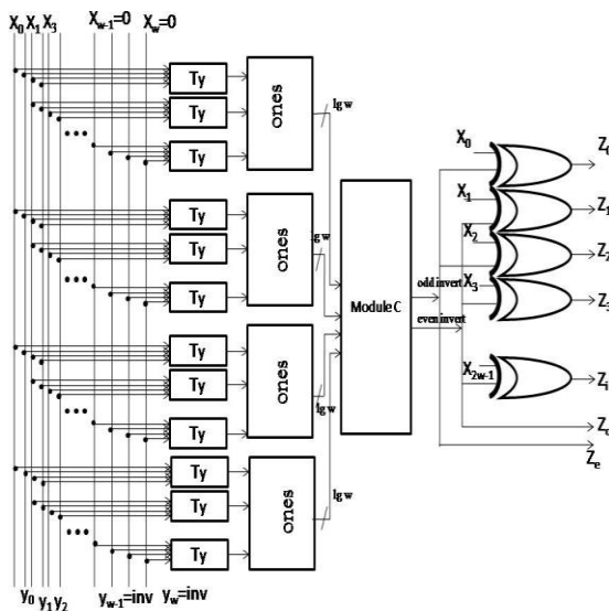
Fig.3. Encoder Architecture Scheme III.
