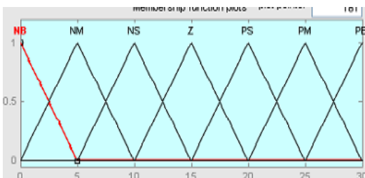
Fig.15.Output membership function
