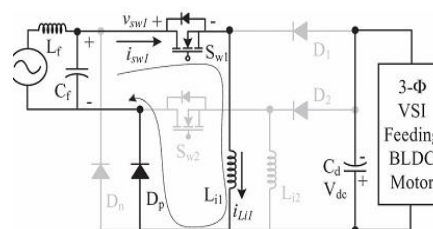
Fig.6. mode 1 operation
