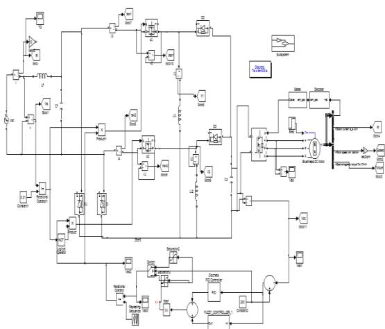
Fig.22.Simulink circuit for proposed system by using fuzzy controller
