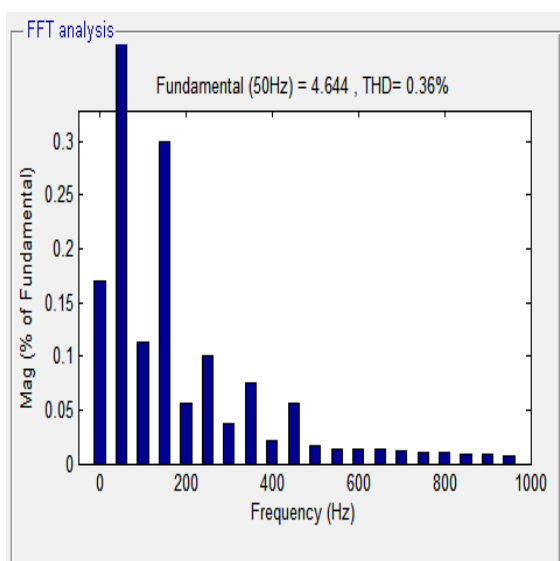
Fig.24.FFT analysis by using fuzzy controller
