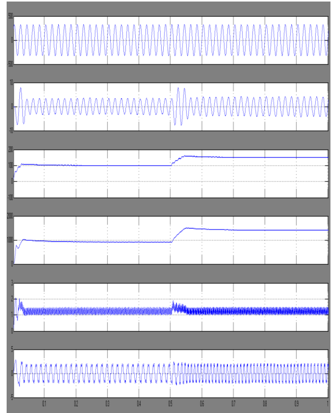
Fig.20.Simulation result of dynamic performance of proposed system during Step voltage variation.
