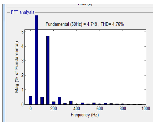
Fig.23.FFT analysis by using PI controller
