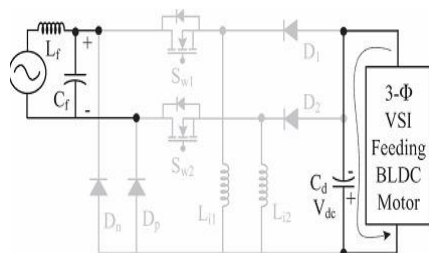
Fig.8. mode 3 operation
