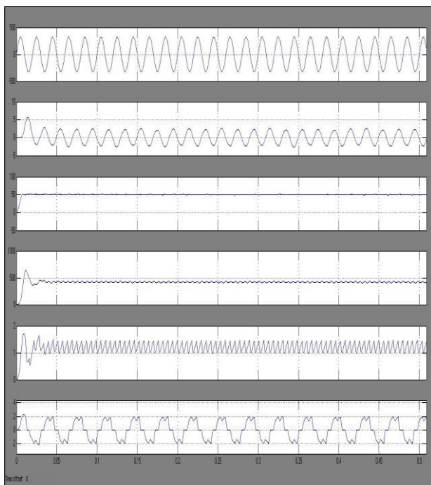
Fig.18.Simulation results for i_{Li1} , i_{Li2} , V_{sw1} , i_{sw1} , V_{sw2} , i_{sw2} of PFC converter under steady state performance
