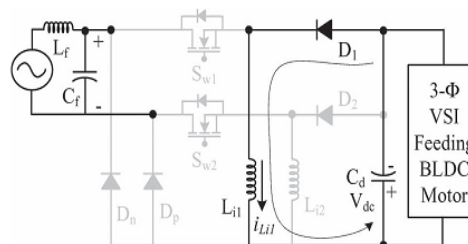
Fig.7. mode 2 operation
