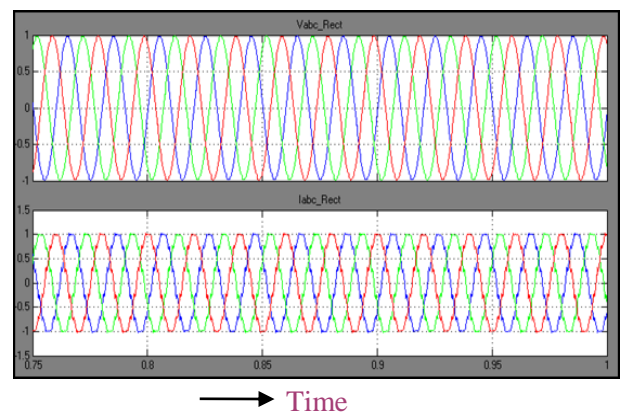
Fig 6. Rectifier side AC Voltage and AC Current
