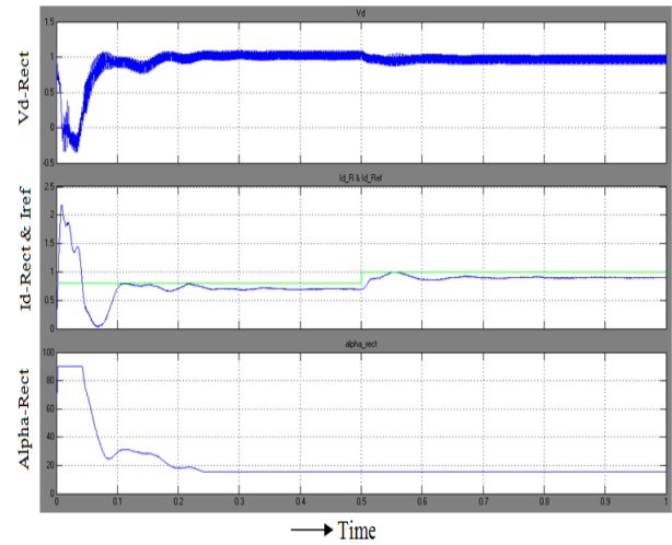
Fig 14. Rectifier side DC Voltage, DC Current and firing angle order with ANN
