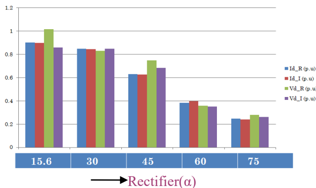
Fig 16. Effect due to change in Rectifier firing angle (chart representation) using ANN
