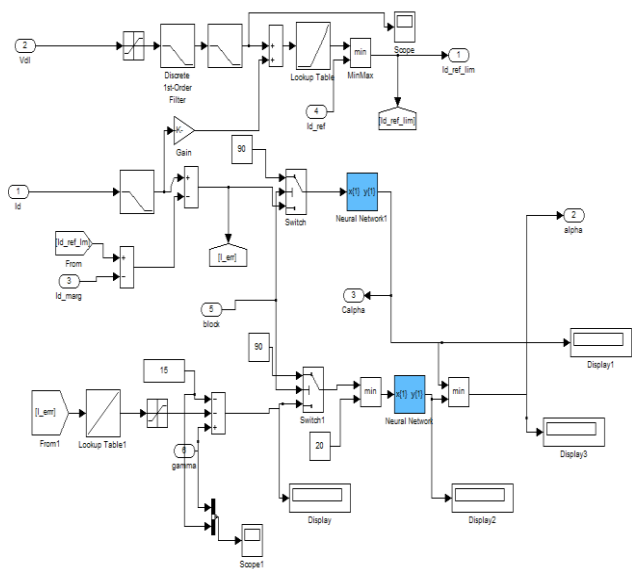
Fig 13. Inverter control with ANN
