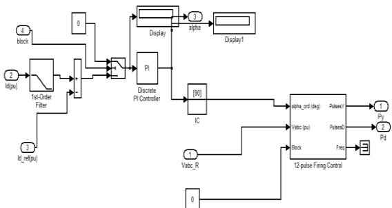
Fig 3. Rectifier control with PI.
