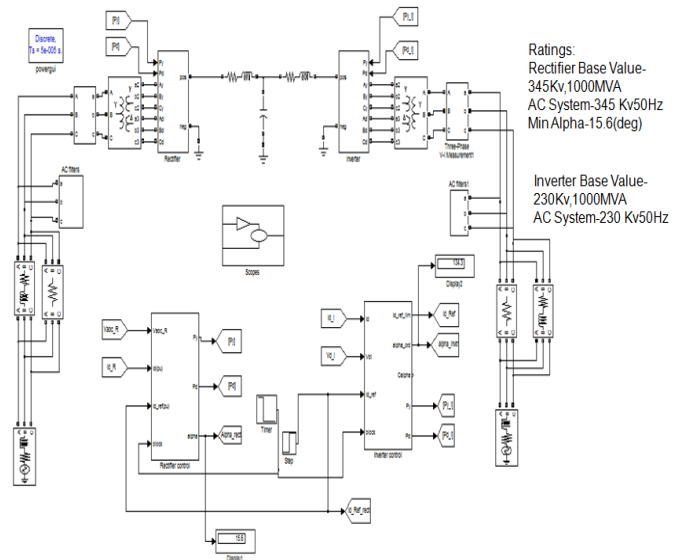
Fig 5. Simulink model of HVDC System
