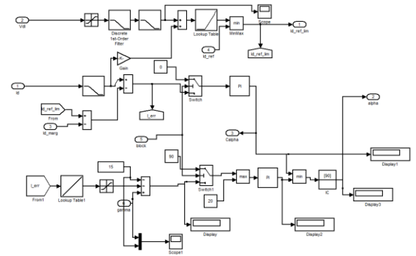
Fig 4. Inverter control with PI.
