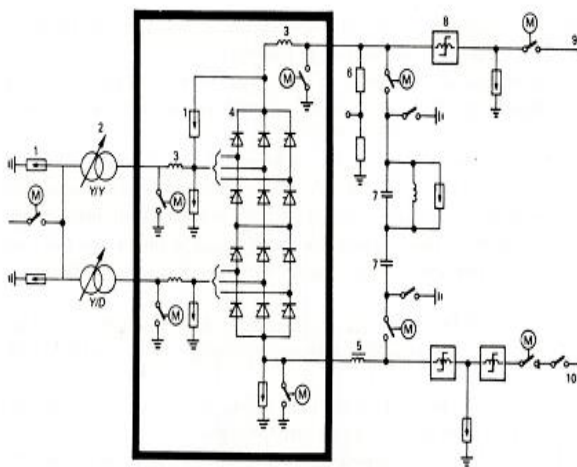
Fig2 The Main Circuit Diagram for One Pole of a Converter Station.
