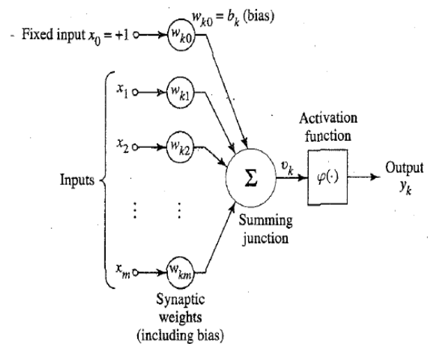
Fig10. Artificial Neural Networks
