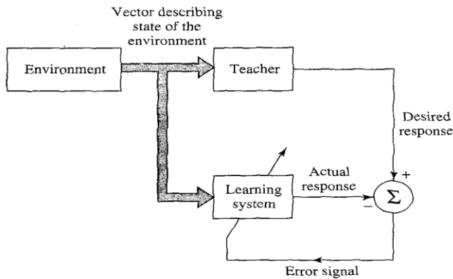
Fig11. Supervised training
