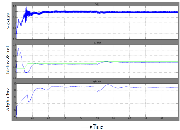
Fig 15. Inverter side DC Voltage, DC Current and firing angle order with ANN
