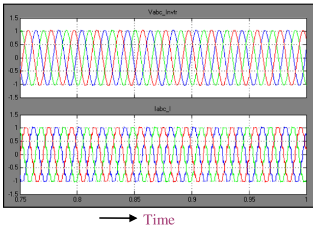
Fig 7. Inverter side AC Voltage and AC Current
