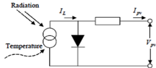
Photovoltaic cell equivalent circuit
