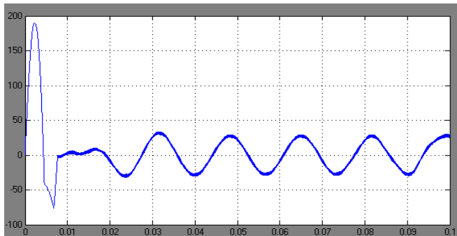
Figure 13: Single phase source current with hysteresis technique using PI controller
