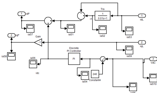
Figure 11: Simulink Model of PI controller based APF
