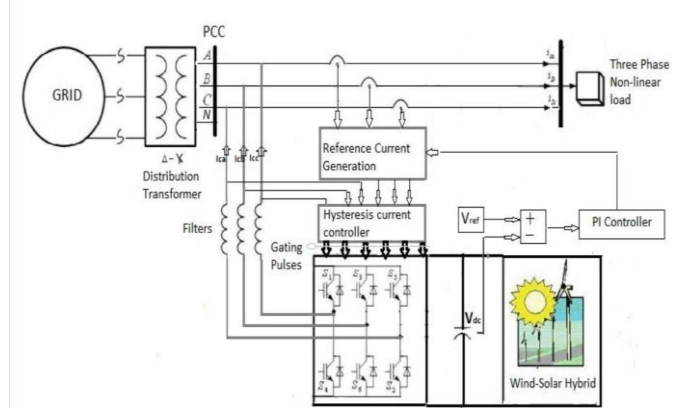
Figure 3: control block diagram of hysteresis controlled APF
