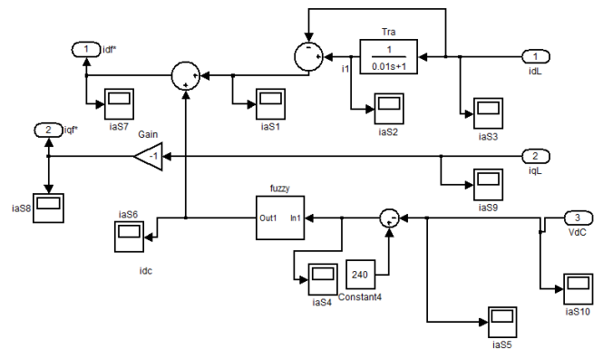
Figure 12: Simulink Model of fuzzy controller based APF
