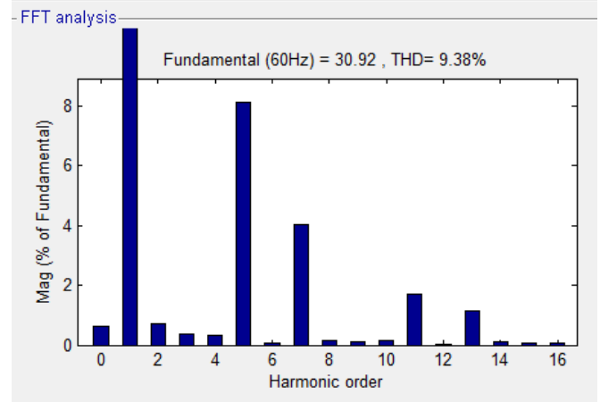
Figure 14: THD without active filter
