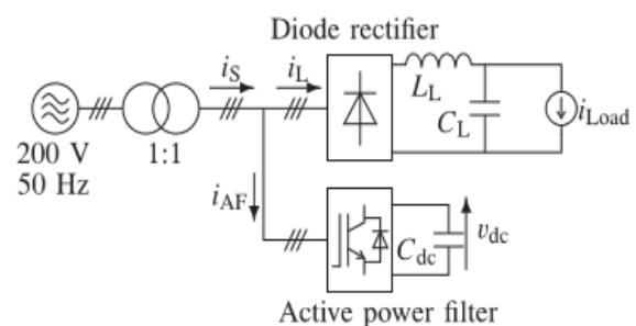
Figure 1: Block diagram of proposed APF
