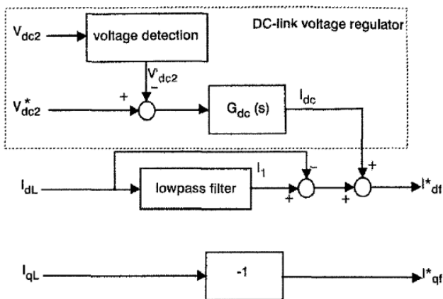
Figure 4: Block diagram of d- and q-axis reference current of active power filter
