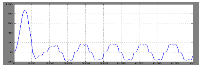
Figure 13: Source current without filter
