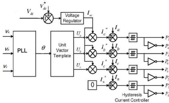
Figure 7: control scheme of the model
