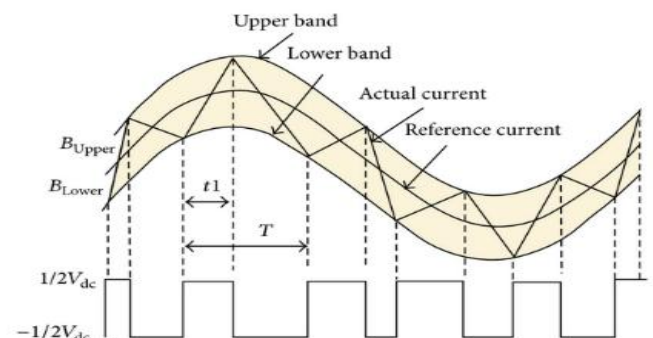
Figure 6: hysteresis current controller
