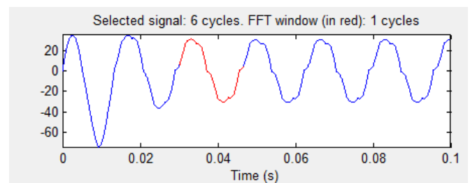
Figure 13: Source current without filter
