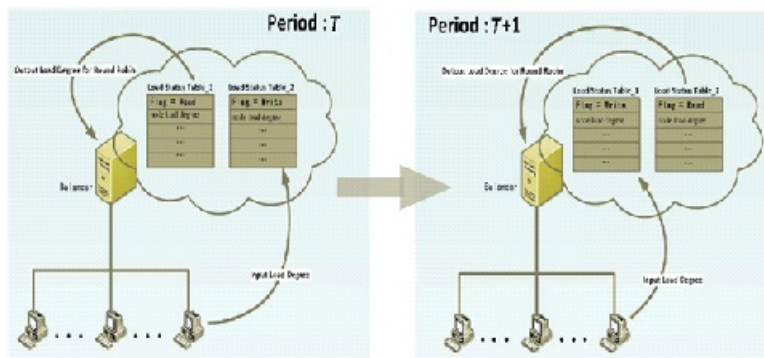
Fig. 4 The solution of inconsistently problem
