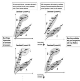
Fig. 2 Differences in data grouping and prediction model search methods between heterogeneous mixture learning and previous techniques.
