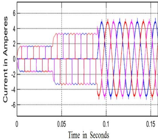
Fig 11. Source Current With Filter
