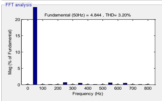
Fig 12 Thd Of Source Current After Compensation
