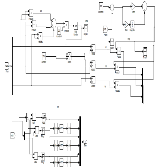
Fig 8. Hystersis With Pi Controller
