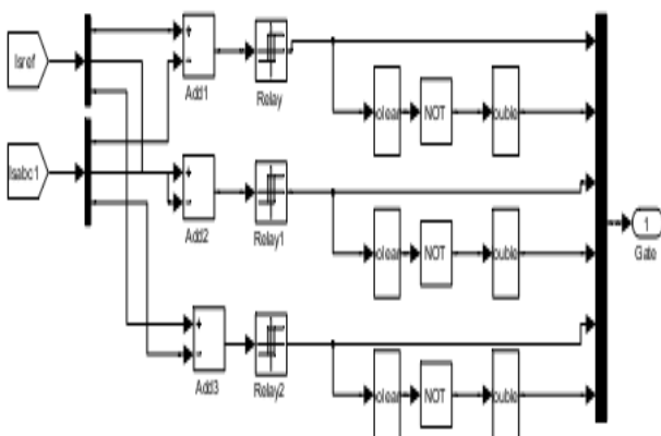
Fig. 4: Simulink Model of Hysteresis Current Control
