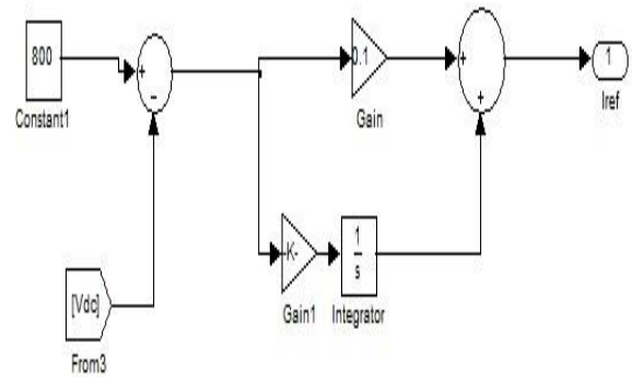
Fig.5: MATLAB Simulink model of PI control
