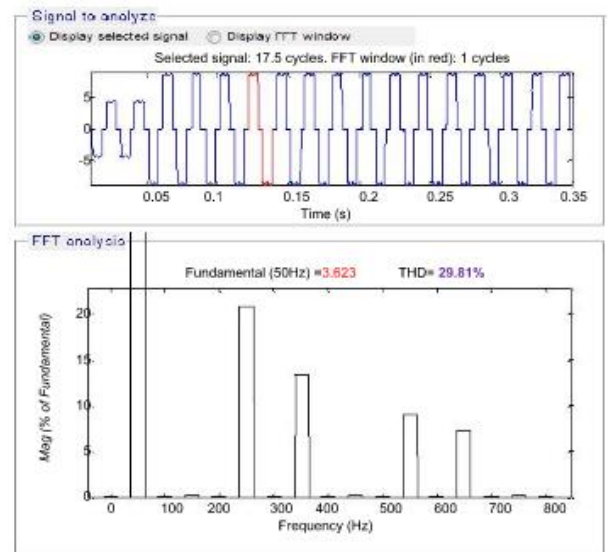
Fig 10. THD of Source Current Before Compensation
