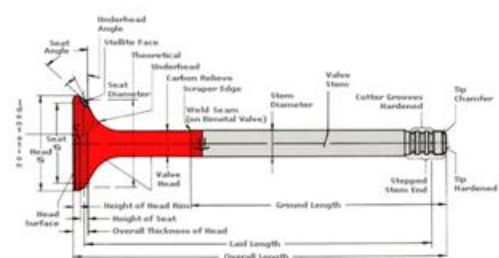
Figure 1.2 dimension of typical valves
