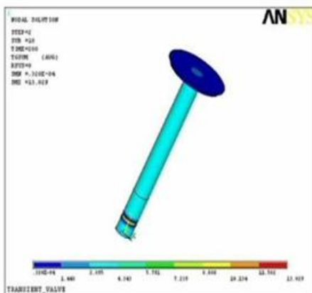
Figure.6.3. Thermal Flux results in ANSYS.
