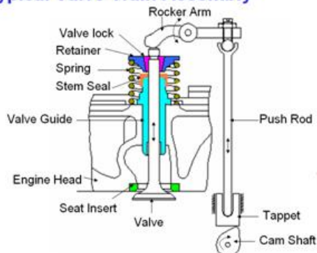
Figure 1.1 typical valve train assembly
