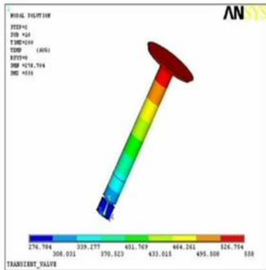
Figure.6.1. Temperature in ANSYS.
