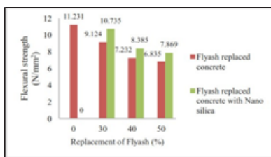
Flexural strength comparison for 28 days
