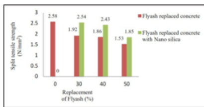
Split tensile strength comparison for 28 days
