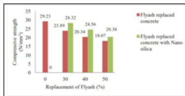
Compressive strength comparison for 28 days
