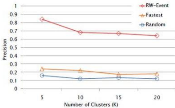
Figure 1: Precision @ K for our classifier and baselines.
