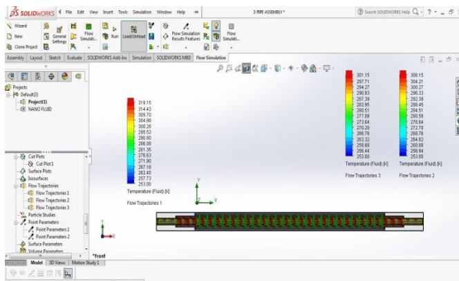
Fig: 10 Flow trajectories of three fluids
