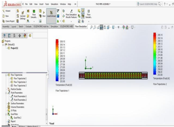
Fig:8Flow trajectories of hot and cold fluid
