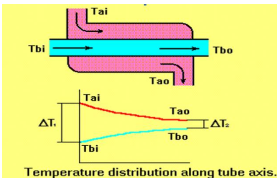
Fig: 1 Parallel flow Heat Exchanger
