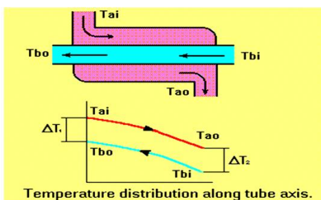
Fig: 3 counter flow heat exchanger
