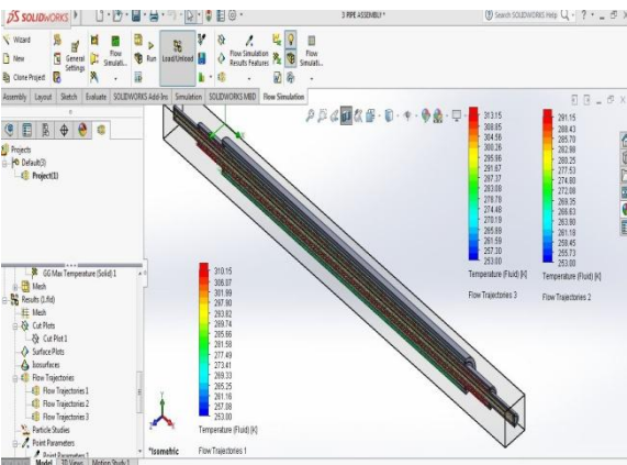
FIG:9Flow trajectories of three fluids
