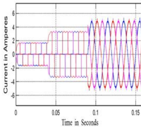
Fig 11. Source Current With Filter
