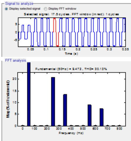
Fig 10. THD Of Source Current Before Compensation
