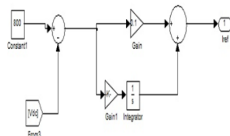
Fig.5: MATLAB Simulink model of PI control
