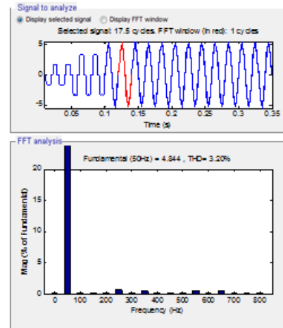
Fig 12 Thd Of Source Current After Compensation
