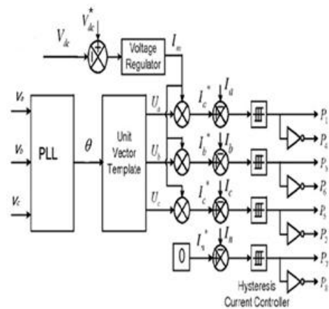
Fig 2:Control scheme
