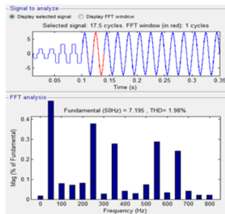
Fig 15 THD Of Source Current With fuzzy
