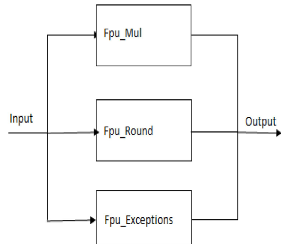
Figure 3. Multiplier structure with rounding and exceptions
