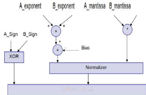
Figure 2. Multiplier structure.
