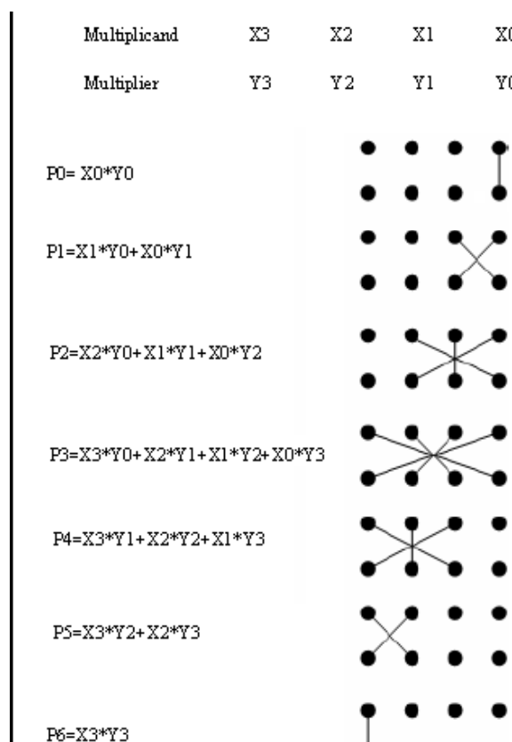
Fig 5: 4 by 4 Vedic Multiplier.
