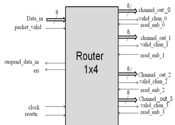
Figure1: Block Diagram of Router Protocol III. Operation
