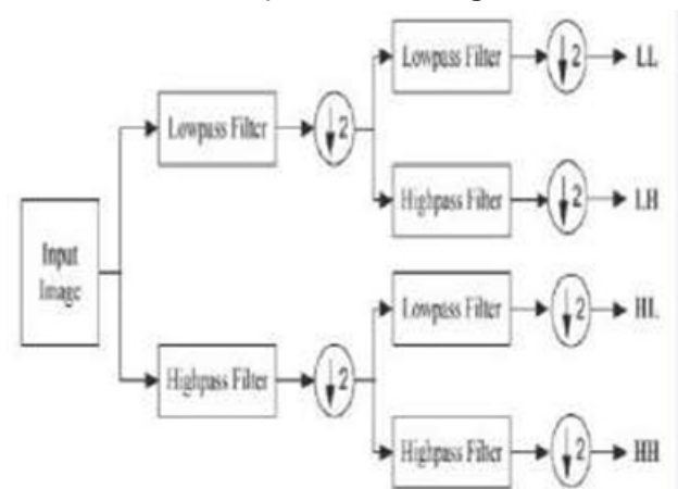
Fig.4 Block diagram of Discrete Wavelet transform
