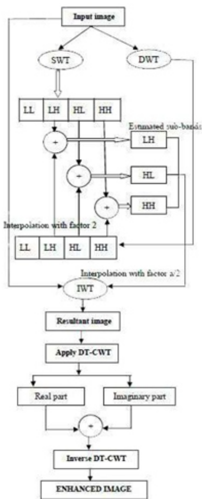
Fig.5 Block diagram of proposed work.
