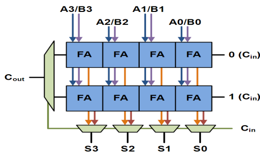
Figure 1: Basic carry Select adder.
