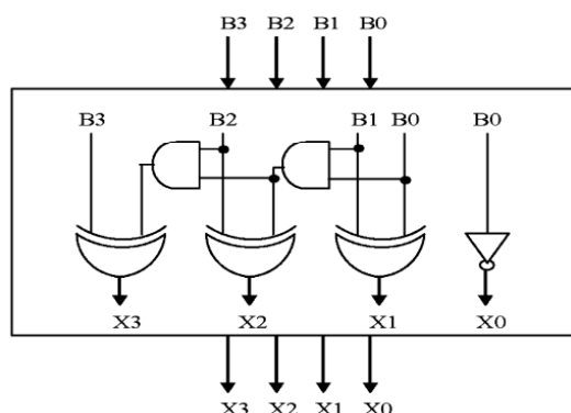
Figure 1: 4 Bit BEC.
