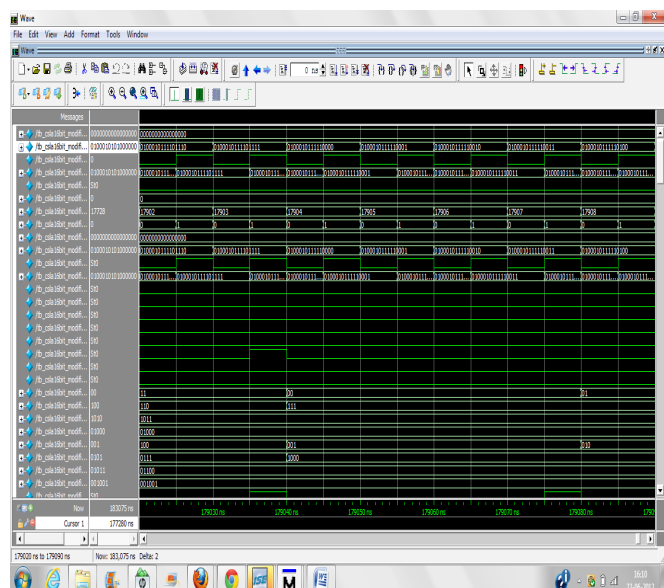
Figure. 8. Modified 16-bit CSLA
