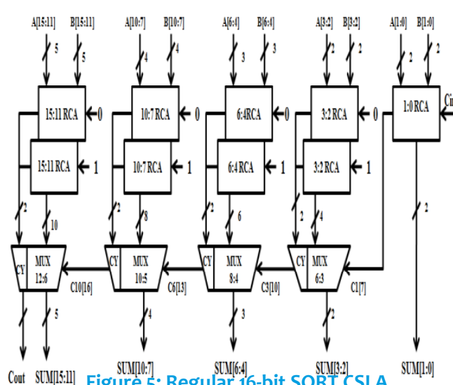
Figure 5: Regular 16-bit Sqrt CSLA
