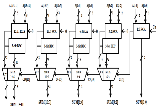
Figure 6. Modified 16-bit SQR CSLA.
