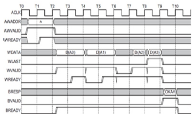
Figure 1: Write address and data burst.
