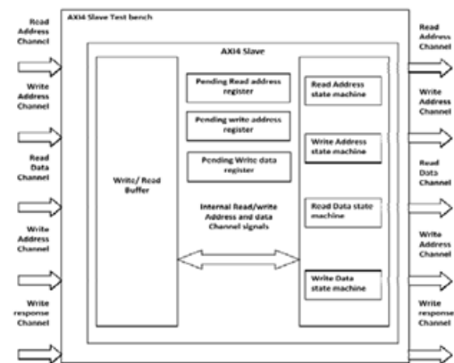
Figure 4: AMBA AXI slave Read/Write block Diagram
