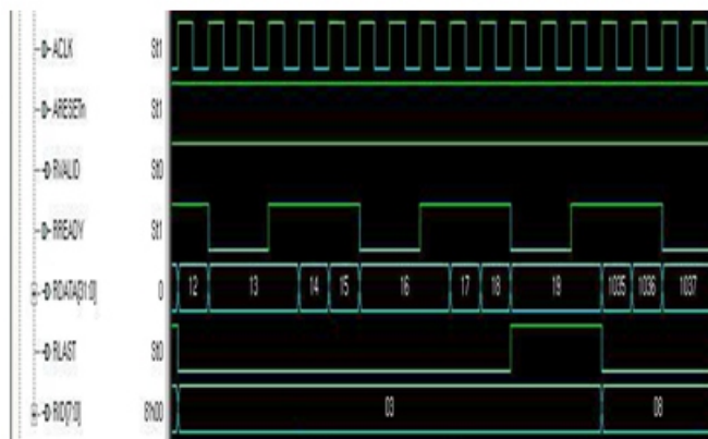
Figure 12: Simulation result of slave for single read data operation.
