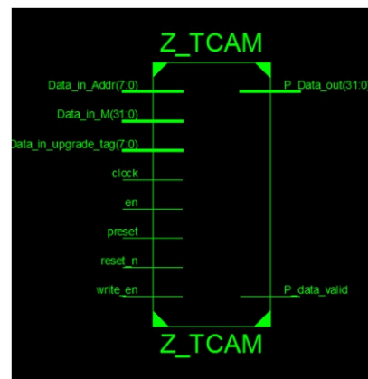
5.1.Z-TCAM block diagram
