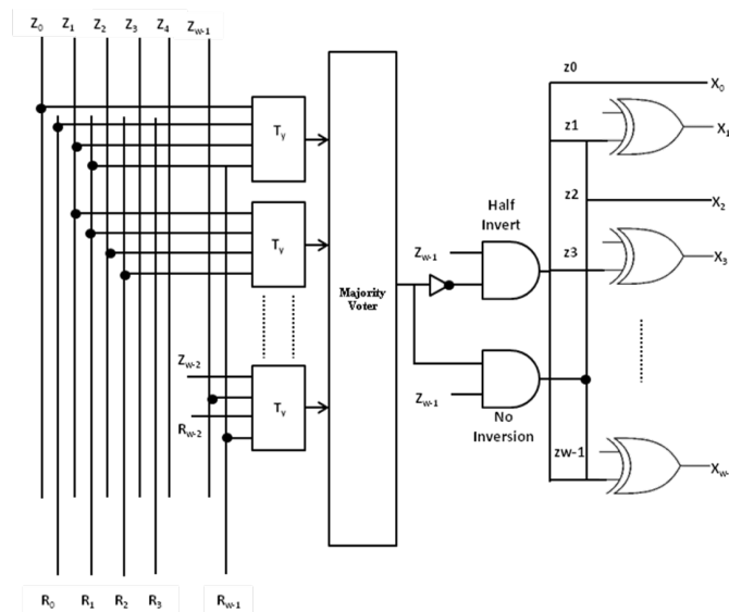
Fig.5. Decoder Architecture Scheme 1.
