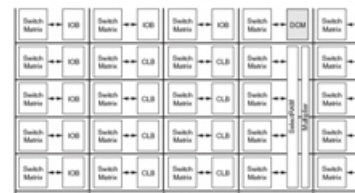
Fig. 1. Routing Resources
