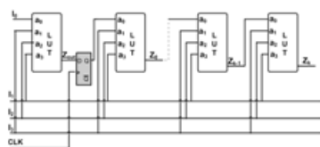
Fig. 6. Proposed configuration of BUT
