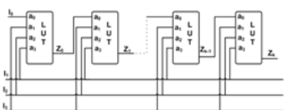
Fig. 7. Configuration of BUT to detect short delay fault
