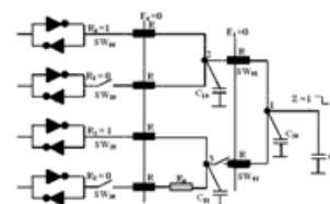
Fig. 4. 2-input LUT with resistive open
