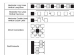
Fig. 2. Hierarchical Routing Resources
