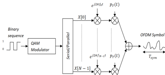
Fig.1 Multi-Carrier Modulation
