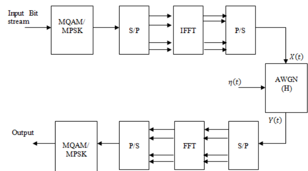
Fig. 3 DFT based OFDM system
