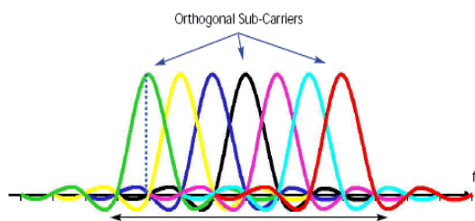
Fig.2 Overlapped frequency in OFDM
