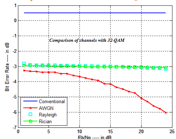
Fig.9 BER performance of proposed and conventional system with 32-QAM under AWGN, Rayleigh and Rician channels
