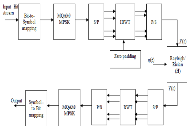
Fig. 5 DWT based OFDM system with Rayleigh and Rician channels
