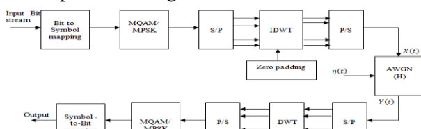
Fig.4 DWT based OFDM system with AWGN channel
