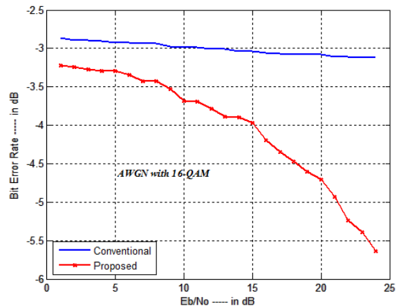
Fig. 7 BER performance of proposed and conventional schemes with AWGN and 16-QAM
