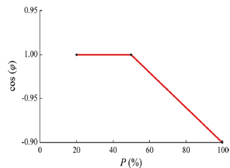
Fig. 6 Reactive power management \cos(\phi) = f(P)
