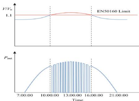
Fig. 2 Repeated network disconnections due to overvoltage
