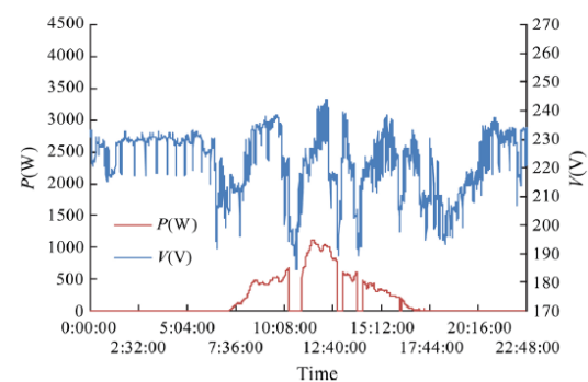
Fig. 4 Daily voltage & power fluctuations—cloudy day
