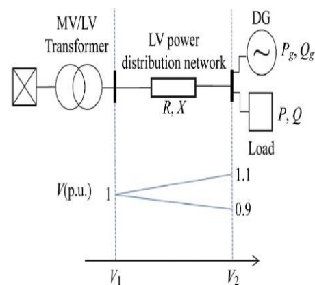
Fig. 1 Voltage rise effects in radial weak distribution networks
