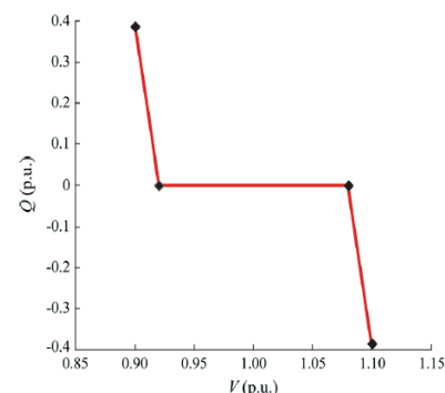
Fig. 7 Reactive power management for voltage regulation
