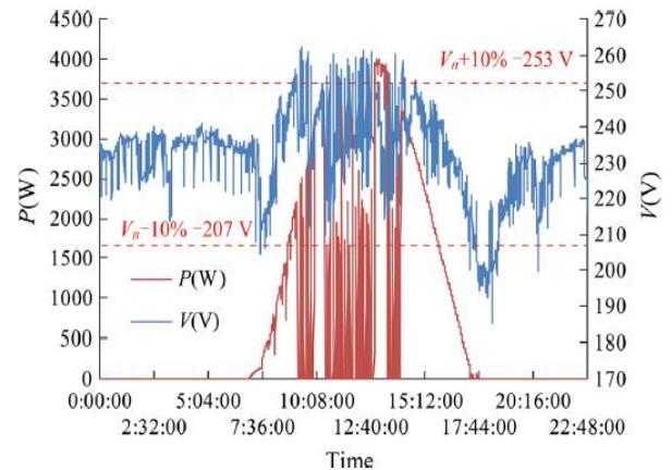
Fig. 3 Daily voltage fluctuations and disconnections—sunny day
