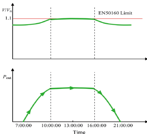
Fig. 5 Active power curtailment for voltage smoothing
