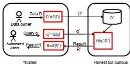
Fig. 1. The system architecture for RASP-based query services.
