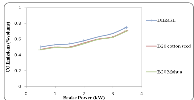
Figure 6: The variation of CO emissions with brake power
