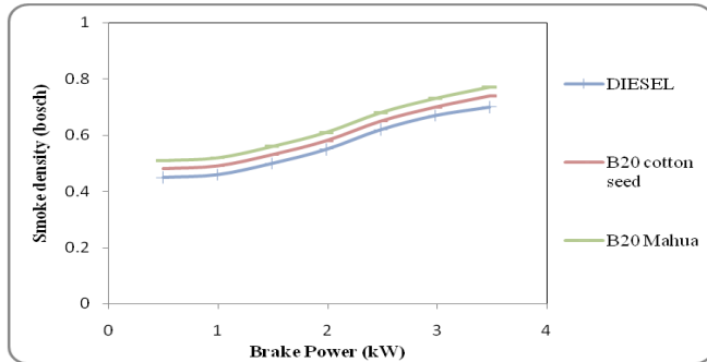
Figure 4: The variation of Smoke density with power output
