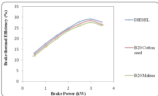
Figure 1: The variation of Brake thermal efficiency
