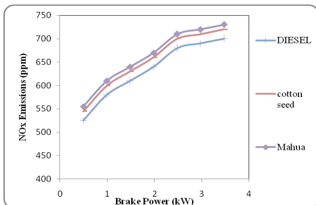
Figure 7: The variation of Nitrogen oxide emissions
