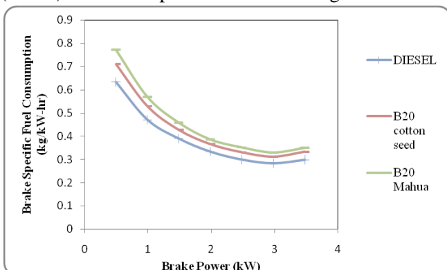
Figure 2: The variation of BSFC with brake power
