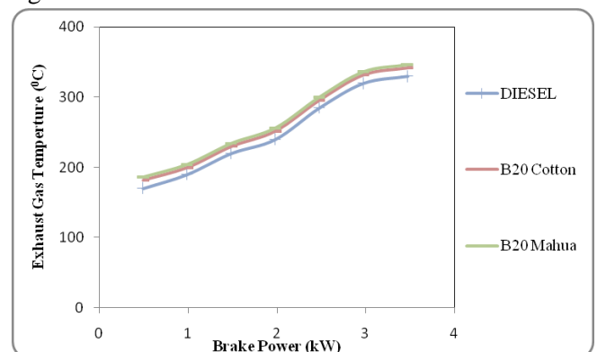
Figure 3: The variation of EGT with brake power
