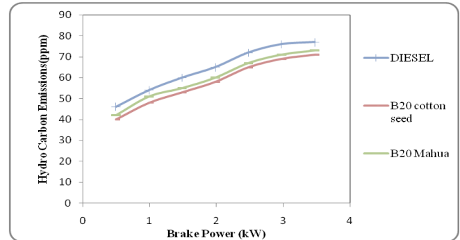
Figure 5: The variation of HC emissions with brake power
