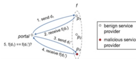
Figure 4: Consistency check.
