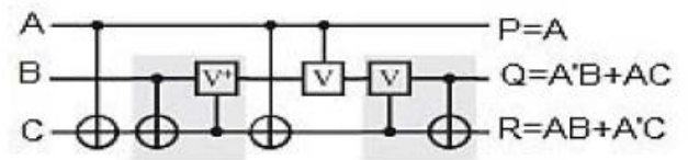
Fig. 2(b) Quantum Representation of Fredkin Gate
