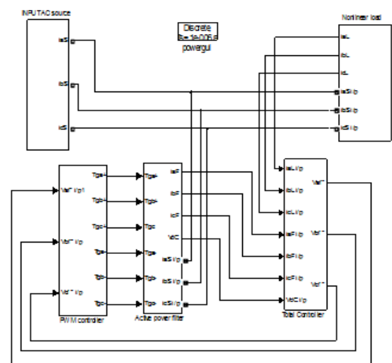
Figure 9: Simulink Model of PWM Controlled APF for the Three-Phase Power System
