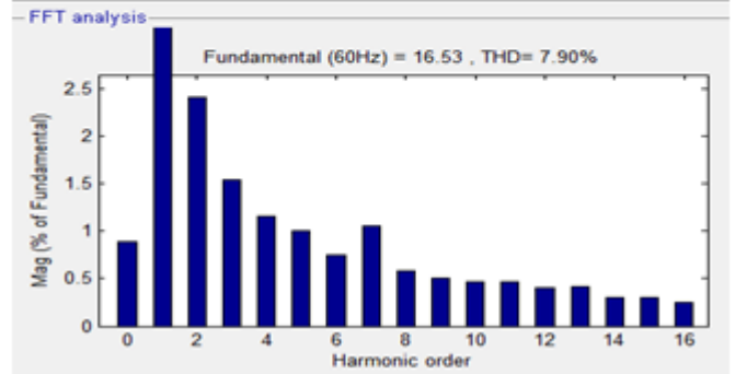
Figure 15: THD with pwm technique
