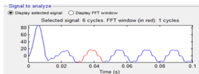
Figure 11: Source current without filter
