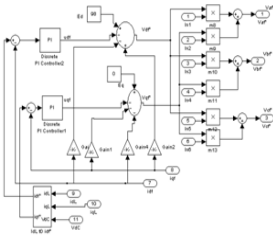
Figure 10: Simulink Model for d and q axis current controllers of APF
