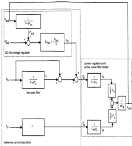
Figure 7: 8 Analytical model for active power filter
