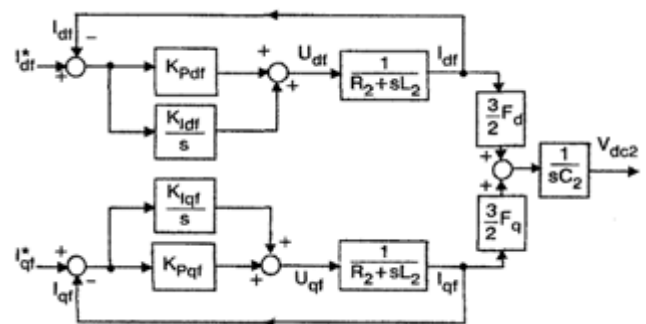
Figure 6: Equivalent control block diagram d- and q-axis current control loops of active power filter.
