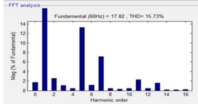
Figure 12: THD without active filter
