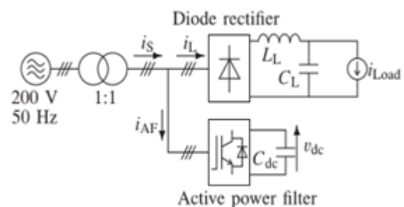
Figure 1: Block diagram of proposed APF
