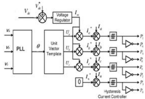
Figure 8: control scheme of the model
