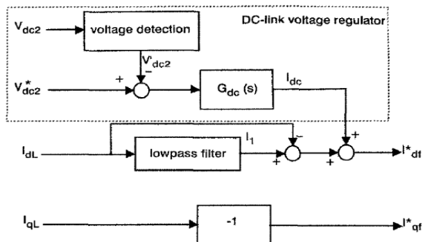
Figure 4: Block diagram of d- and q-axis reference current of active power filter
