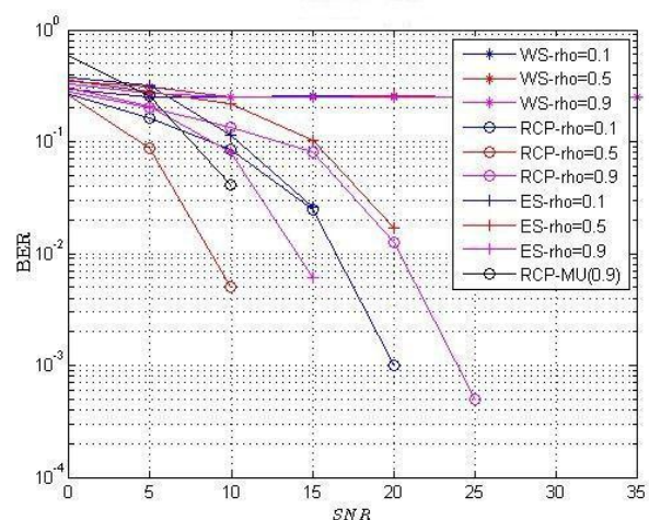
Fig-6: BER performance of RCP
