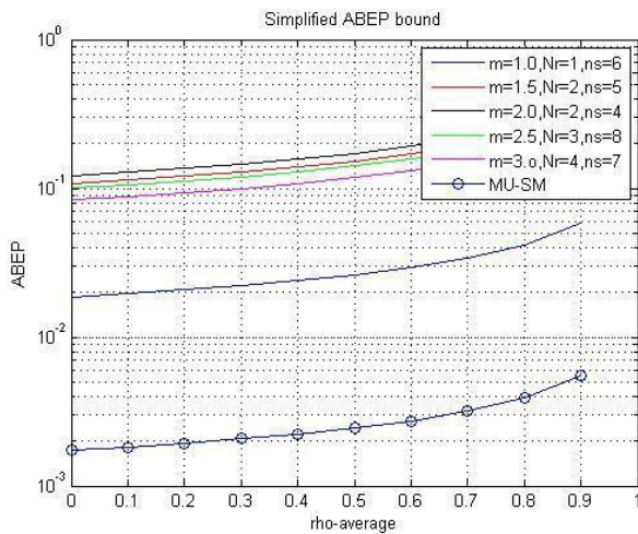
Fig-7: ABEP performance
