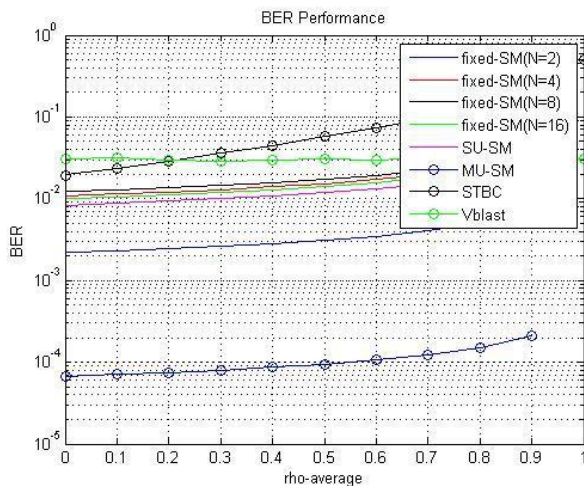
Fig-8: BER Plot
