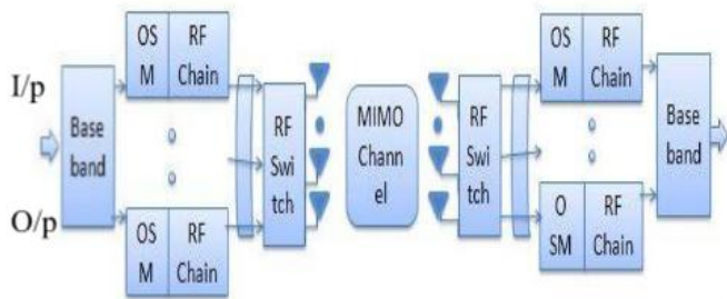
Fig-3: Block diagram of multi stream MIMO.
