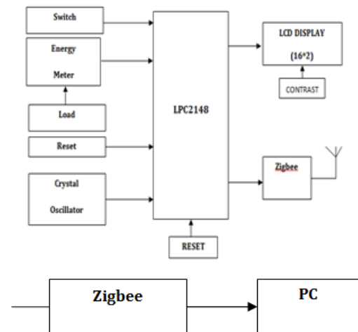
BLOCK DIAGRAM
