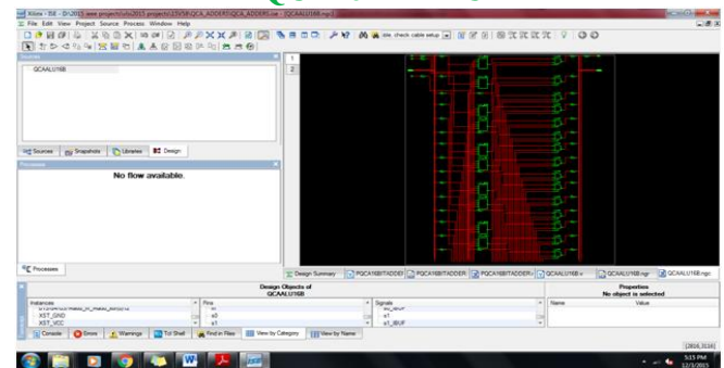
Figure 8.2(c): Technology schematic of Internal block of PQCA16BITALU
