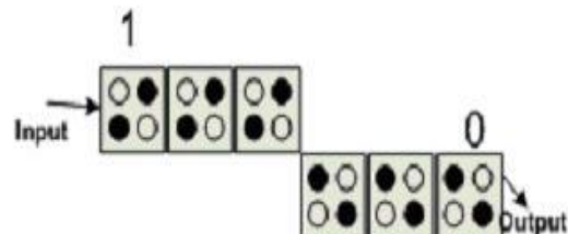
Fig.3. QCA Inverter
