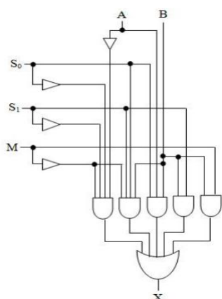
Fig 6: Logic Circuit of Logical Extender
