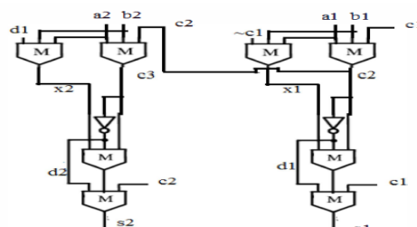
Fig 7.1(a): Modified novel bit adder 1: 2 bit basic module.
