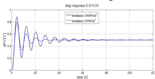
Figure 3: The step response of the under-damped converter.
