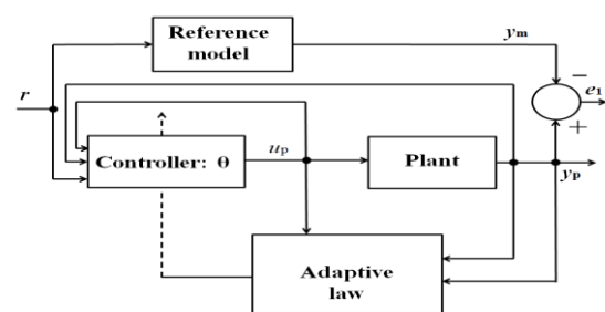
Figure 4: The general scheme of the MRAC structure.
