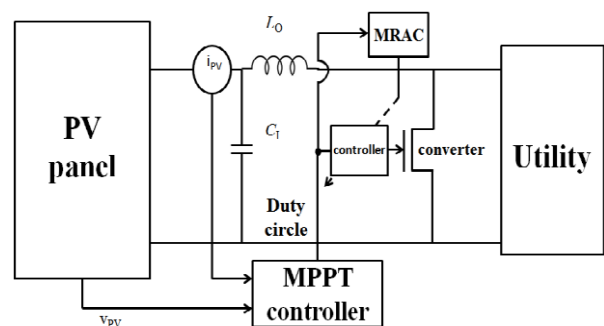
Fig 1: The scheme of entire control system.
