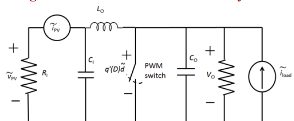
Figure 2: The equivalent small signal circuit of converter.
