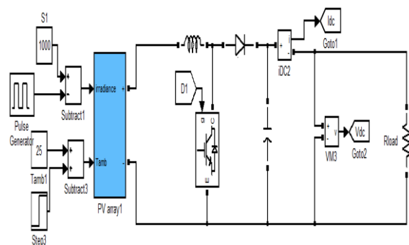
Fig 7: simulation design of proposed converter
