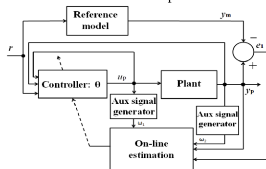
Figure 5: The proposed MRAC in MPPT.
