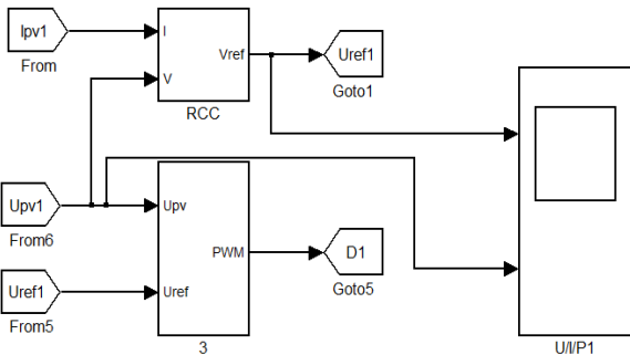
Fig 8: Model Reference Adaptive Control
