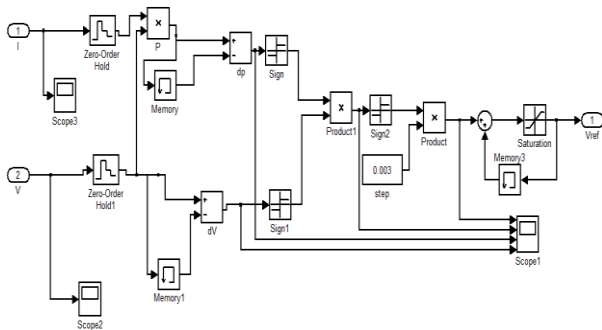
Fig 9: Ripple Co-relation Controller
