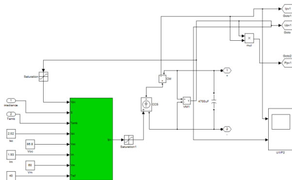
Fig 9: PV-Array
