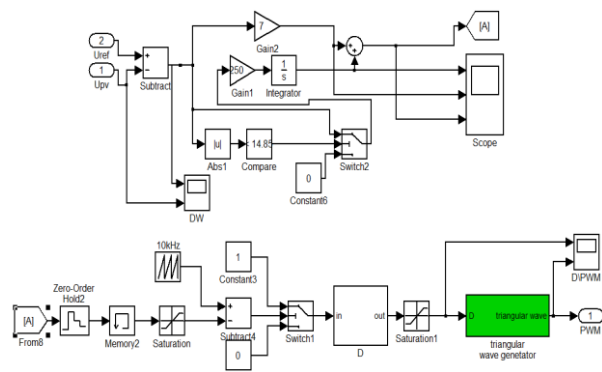
Fig 8: Duty cycle generator
