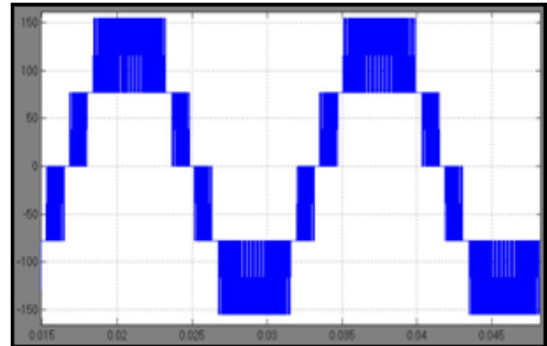
Figure 2: Output voltage of proposed inverter
