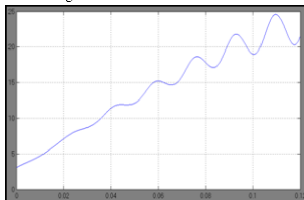
Figure 10: Rotor speed
