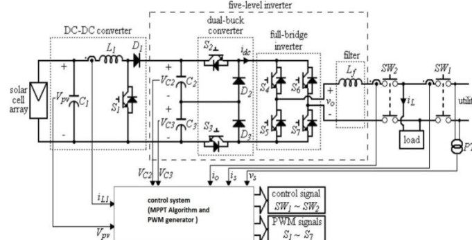
Figure 1: Circuit design of five-level inverter interfaced with PV energy conversion system
