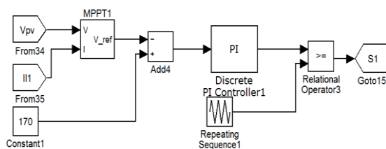
Figure 3: MPPT controller
