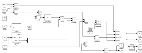
Figure 4: inverter control circuit
