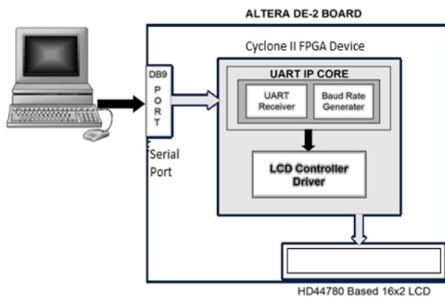
Fig. 3 Application design of UART
