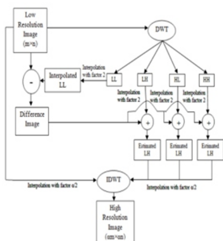
Fig2. Existing DWT-RE block diagram
