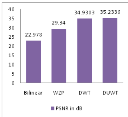
Fig7. Comparison of PSNR values
