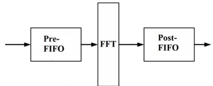
Figure 5: Proposed synchronizer using Pre-FIFO and POST-FIFO
