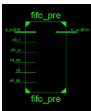
Figure 9: Block Diagram for Pre-FIFO
