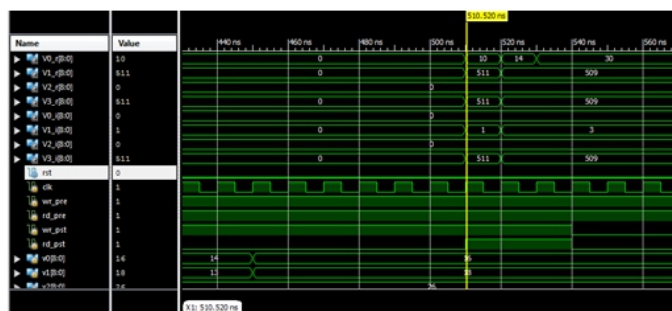
Figure 15: Simulation for LTE
