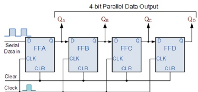
Figure 3: Serial-in Parallel Out
