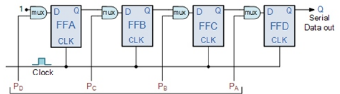
Figure 4: Parallel-in Serial Out
