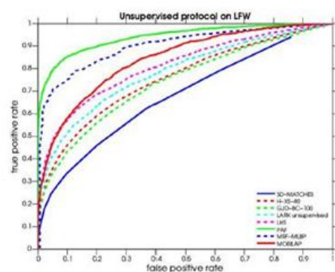
ROC curves of different approaches on the LFW dataset for the Unsupervised protocol.
