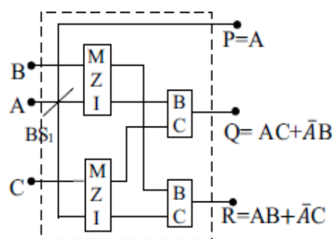
Fig. 2(b): MZI based optical implementation of Fredkin gate
