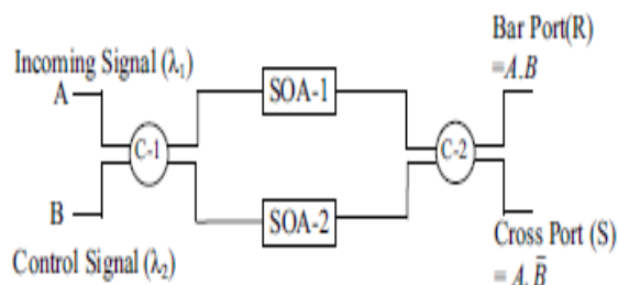
Fig. 1: Semiconductor Optical Amplifier based MZI Switch
