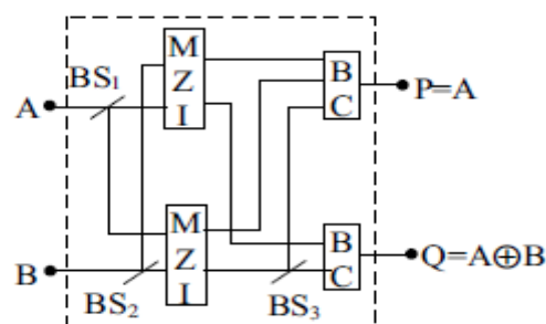
Fig. 2(a): MZI based optical implementation of Feynman gate
