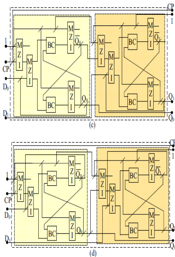
Fig. 3: Design of all optical reversible (a) asynchronous positive edge-triggered down counter, (b) asynchronous positive edge-triggered up counter (c) asynchronous negative edge-triggered down counter (d) asynchronous negative edge-triggered up counter using MZI switch.
