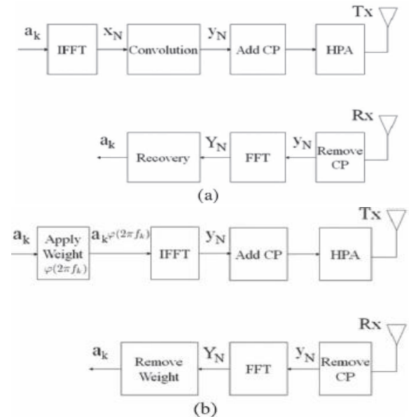
Fig.1. Simplified block diagrams for an OFDM system with (a) convolution scheme and (b) proposed weighting scheme.
