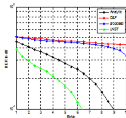
Figure 4.3: OFDM performance in terms of BER
