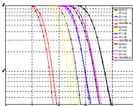
Figure 4.1: Results for different number of symbols N=128, 256, 512
