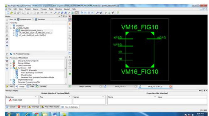
Figure 7.13: RTL schematic of Top-level Vedic Multiplier Modified square root Carry Select Adder
