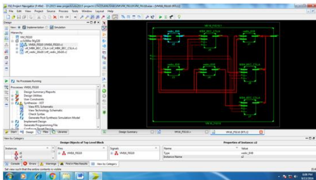
Figure 7.14: RTL schematic of Internal block Vedic Multiplier Modified square root Carry Select Adder
