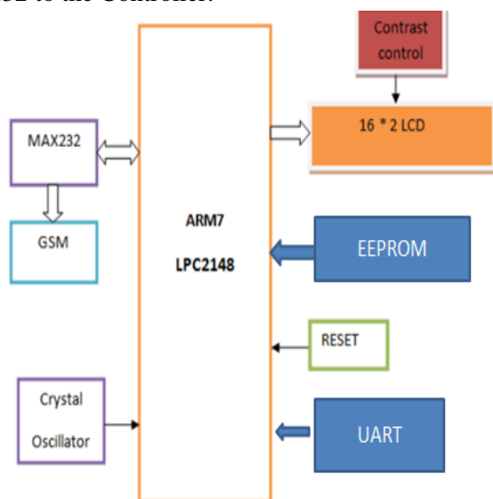
Fig 1 Block Diagram
