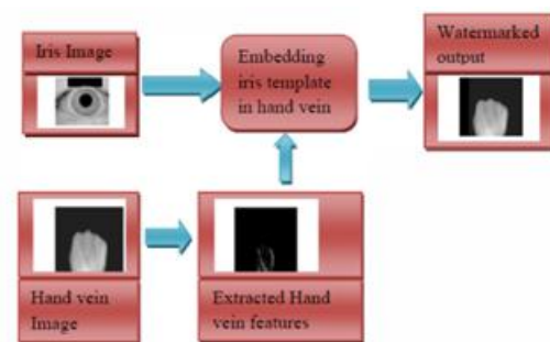
Fig. 1. Watermark Embedding
