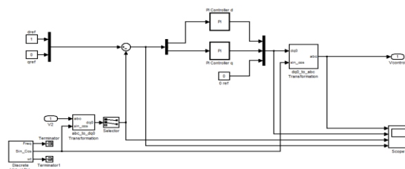
Figure 10. MATLAB based model of the proposed control method
