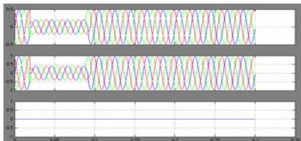
Figure 15. Without dynamic voltage restorer source voltage and injected voltage
