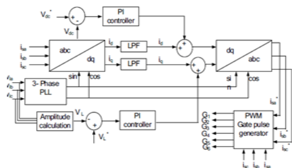
Figure 7. control scheme of the DVR
