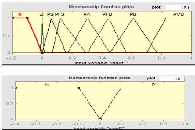
Figure 8. Data for the implemented fuzzy system for DVR.
