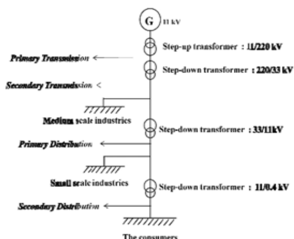
Figure 1. single line diagram of power supply system
