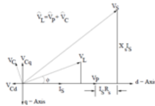
Figure 5: Phasor diagram for the system
