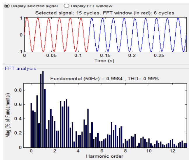
Figure 19. THD with FUZZY controller for both VSCs
