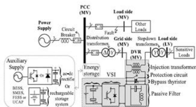
Figure 3. Typical application of DVR in a Medium voltage distribution system
