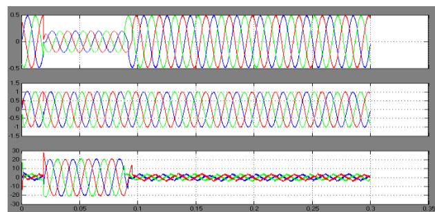
Figure 18. Simulation results using fuzzy controller
