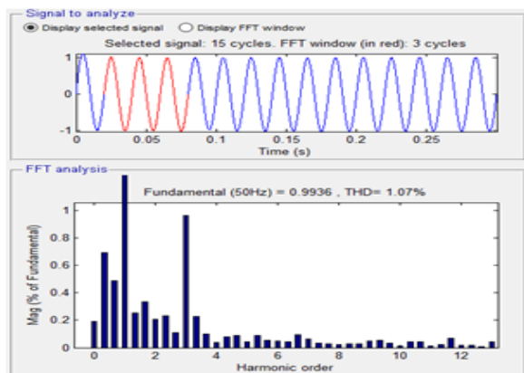
Figure 17. THD for load voltage with PI controller
