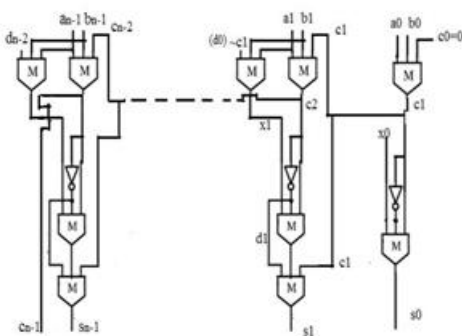
Fig 5(c): Modified novel bit adder I: n bit basic module.
