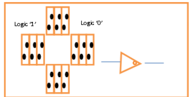
Fig 3: Inverter
