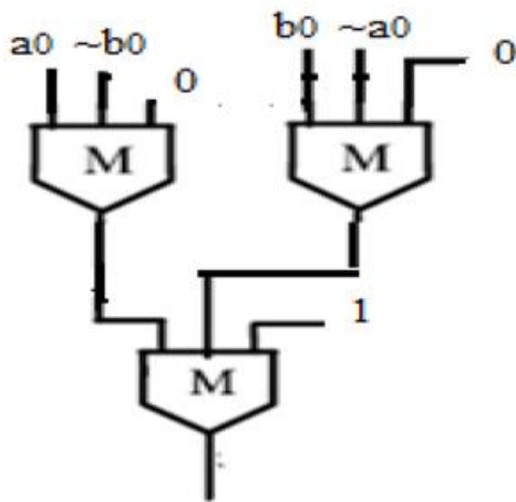
Fig 5(b): Modified novel bit adder 1- Calculation of x0
