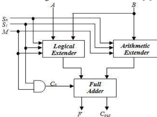
Fig 1: Architecture of ALU
