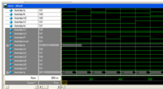
Fig 10 (a): Simulation result of proposed ALU
