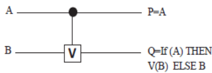
Fig.2. Quantum representation of Controlled-V
