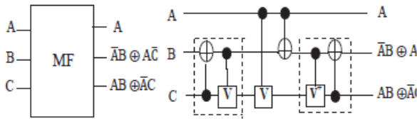
Fig8. MF gate and its Quantum representation
