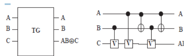
Fig.5. Toffoli gate and its Quantum representation
