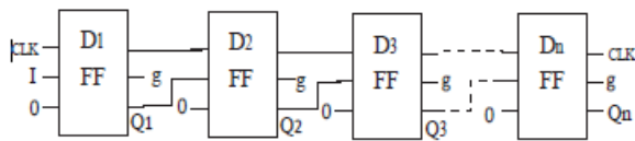
Fig13. Edge-triggered N-bit SISO registers using D-FF
