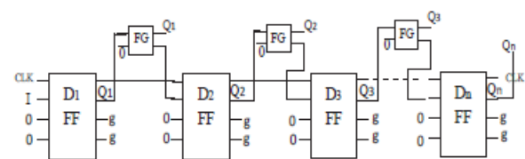
Fig16. Pulse-triggered N-bit SISO registers using master-slave D-FF
