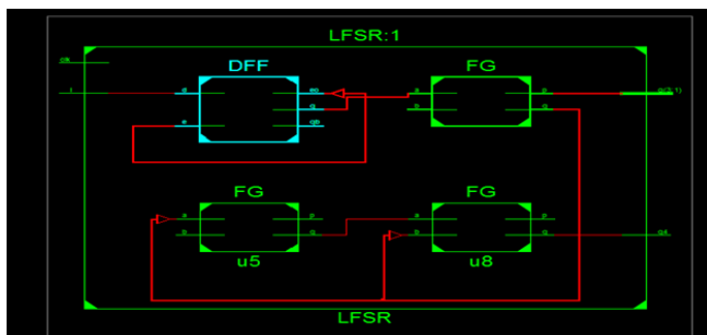
Fig 23. RTL sub schematic of pulse triggered reversible LFSR
