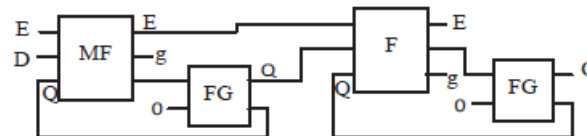
Fig11. Master-Slave D-Ff Using Mf And F Gate
