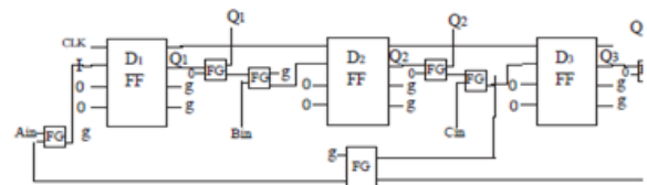
Fig21. Realization of 3 bit Reversible PSA
