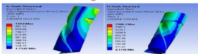
Figure 5.4: Von Mises stress in the case of two flute small end mills
