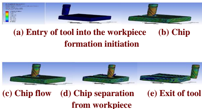
Figure 5.8: Simulation of small burr formation using tool with rake angle 5° and relief angle 6°
