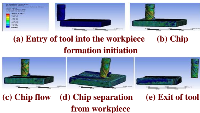
Figure 5.7: Simulation of small burr formation using tool with rake angle 3° and relief angle 8°
