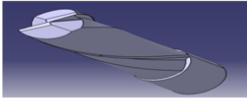
Figure 4.2: CATIA model of two flute small end mill
