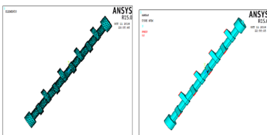
Meshed Model Model with applied load
