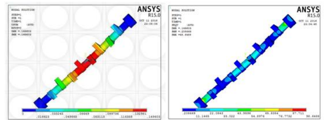
Displacement vector sum Equivalent (Von Mises) Stress
