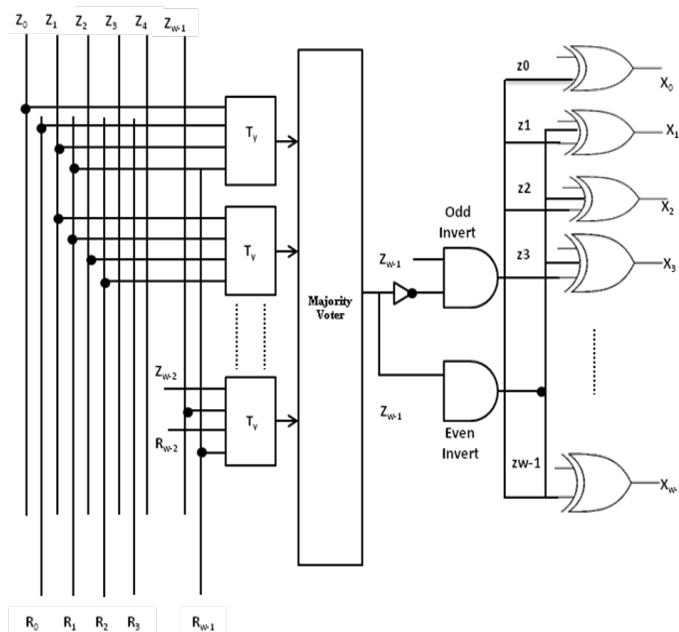
Fig 6: Decoder Architecture Scheme 3.
