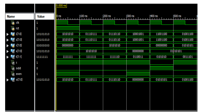
Fig 12: Scheme 3 Decoder
