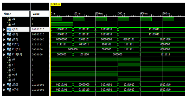
Fig 8: Scheme 2 Encoder
