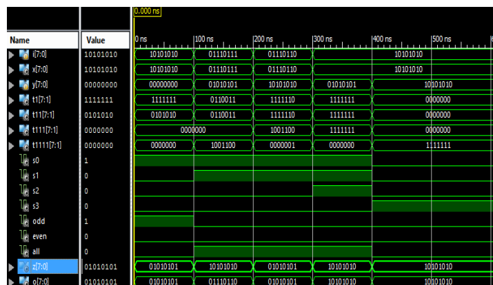
Fig 9: Scheme 3 Encoder
