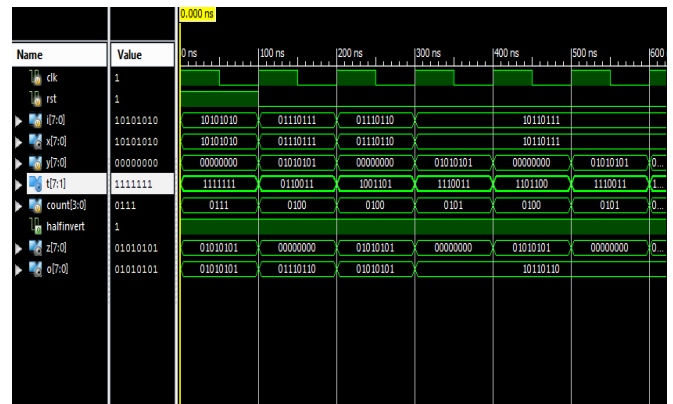
Fig 7: Scheme 1 Encoder
