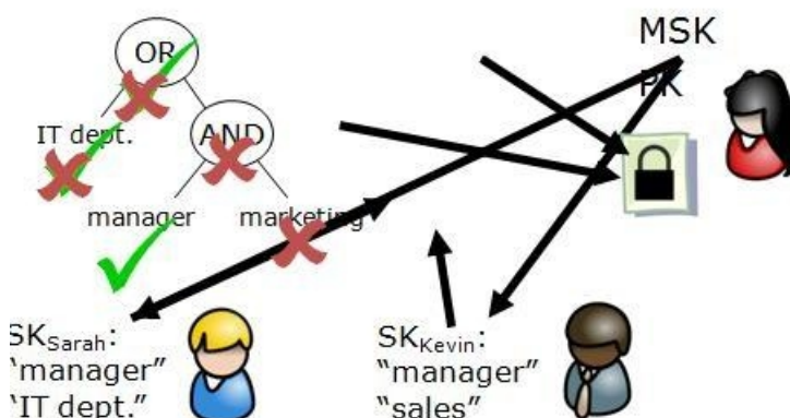
Fig.3.Access Control via Cp ABE
